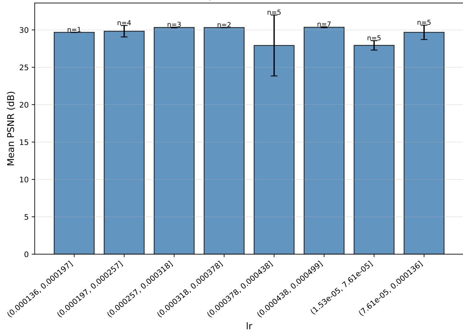
Mean PSNR per value of l_r — SRFormer
